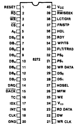
Figure 2. Pin Configuration
