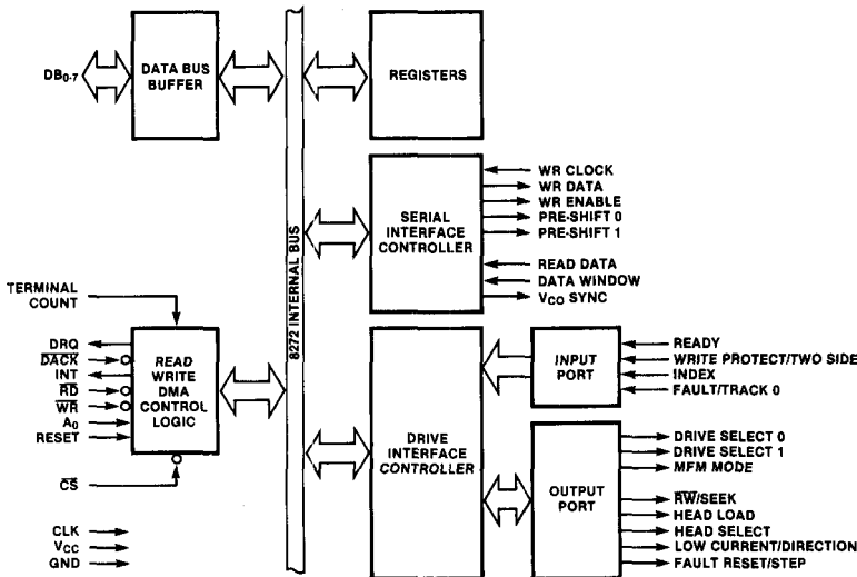
Figure 1. 8272 Internal Block Diagram
